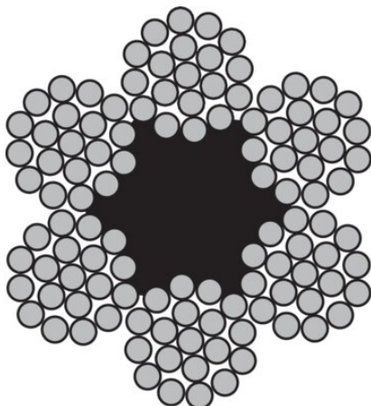
Stropen-kabel
